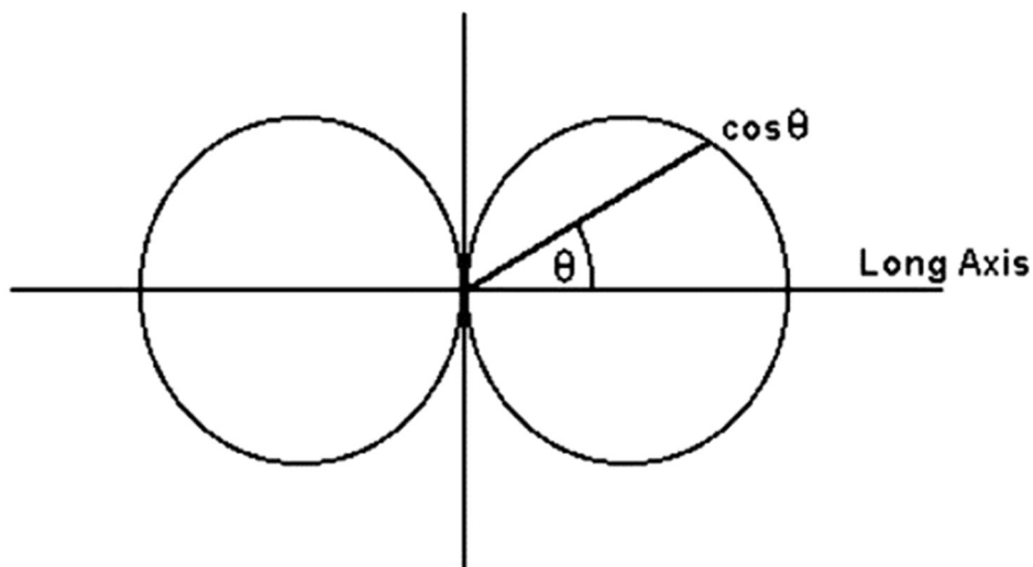
Polar Response of Sensor
