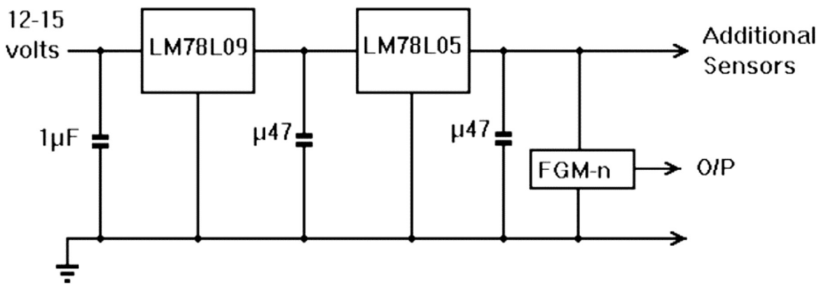
Double Regulation Supply
