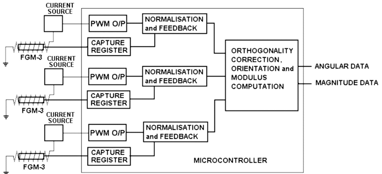
THREE DIMENSIONAL SENSOR SYSTEM
